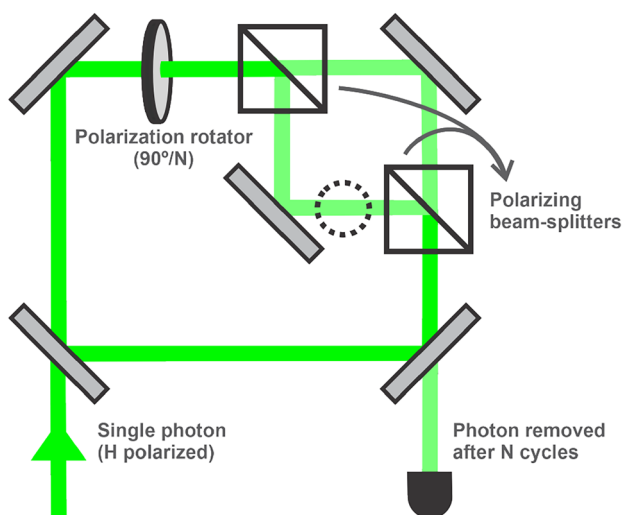
Fig. 3 Variation of the Elitzur-Vaidman bomb testing problem using a cavity for n repetitions of the injected single photon. Adapted from [6]
