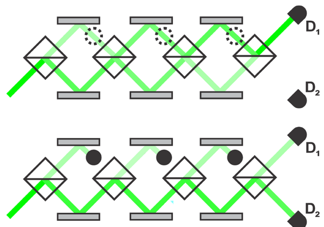
Fig. 4 Variation of the Elitzur-Vaidman bomb testing problem with repeated tests known as interaction-free measurement. Adapted from [5]
