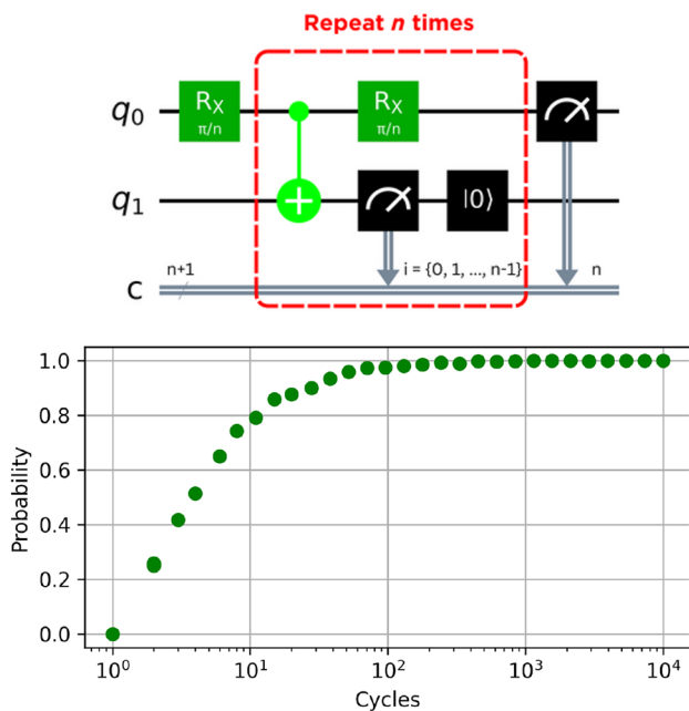
Fig. 8 Quantum circuit for the interaction-free measurement experiment proposed by [5] for n cycles, where R_x(\pi/n) replaces the H gate to control the reflectivity, in which intermediate measurements of qubits representing the state of the bomb q_1 are performed and a final measurement of the photon qubit q_0 ; and experimental data of quantum circuits from 1 to 10,000 cycles using the IBM cloud-based quantum computing service (Qiskit Runtime)
