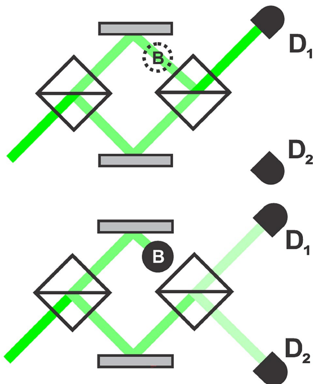
Fig. 1 Elitzur-Vaidman experiment without the bomb (top) and with the bomb (bottom). Adapted from [4]
