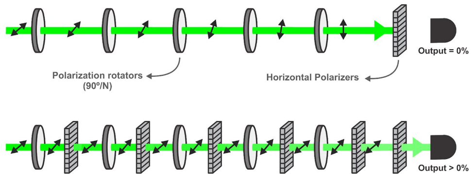
Fig. 2 Horizontal polarization of a photon passing through N polarization rotators (each rotating by 90^\circ/N ) converts it to vertical polarization, leading to its blockage by the horizontal polarizer (top). Inserting a horizontal polarizer after each rotator inhibits the polarization change, allowing detection of light beyond the horizontal polarizer (bottom). Adapted from [9]
