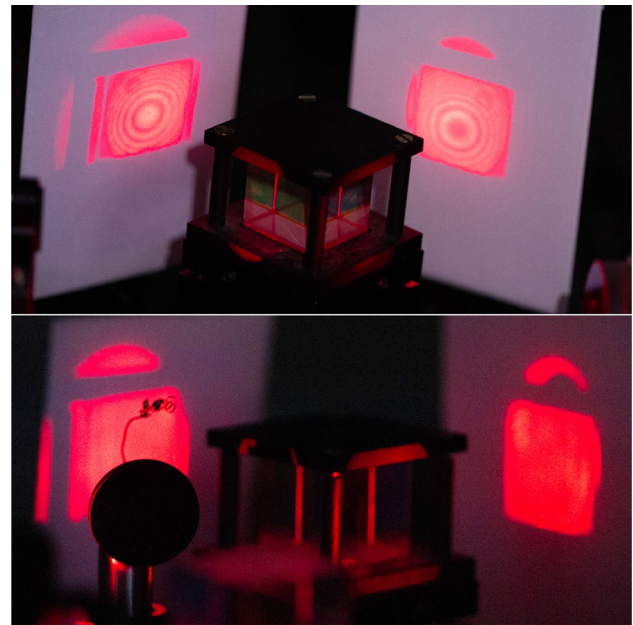
Fig. 6 Comparison between the original EV experiment without an object in the path (top) and with an object in the path (bottom)
