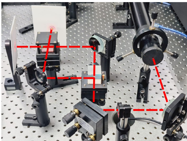
Fig. 5 Reproduction of the original experimental setup of Elitzur-Vaidman bomb testing problem using a Mach-Zehnder interferometer with two 50/50 beam splitters
