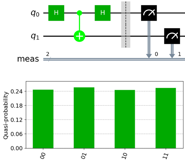
Fig. 7 Quantum circuit for the original EV experiment, using the H gate to represent a 50/50 beam splitter and the C-NOT gate to represent the bomb; and quasi-probabilities of the quantum circuit using the IBM cloud-based quantum computing service (Qiskit Runtime)
